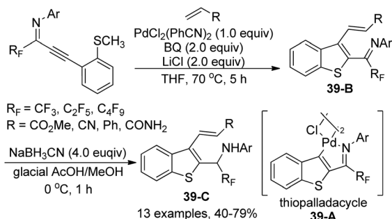
Scheme 39 Synthesis of 3-alkenylbenzo[b]thiophenes.
