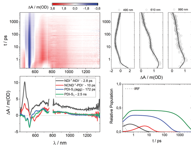
Fig. 6 Top left: Differential absorption 3D map obtained upon fs-TAS of NCND-NDI/PDIs in DMF at room temperature, with 387 nm excitation. Top right: Time absorption profiles and corresponding fittings at 490, 610, and 990 nm. Bottom left: Species associated differential spectra of the \text{NDI}^{\bullet+}\text{-NDI}^{\bullet-} CS state (black), \text{NCND}^{\bullet+}\text{-PDI}^{\bullet-} CS state (red), PDI-centered S_1 (agg) (blue) and PDI-centered S_1 (green). Bottom right: Concentration evolution over time.
