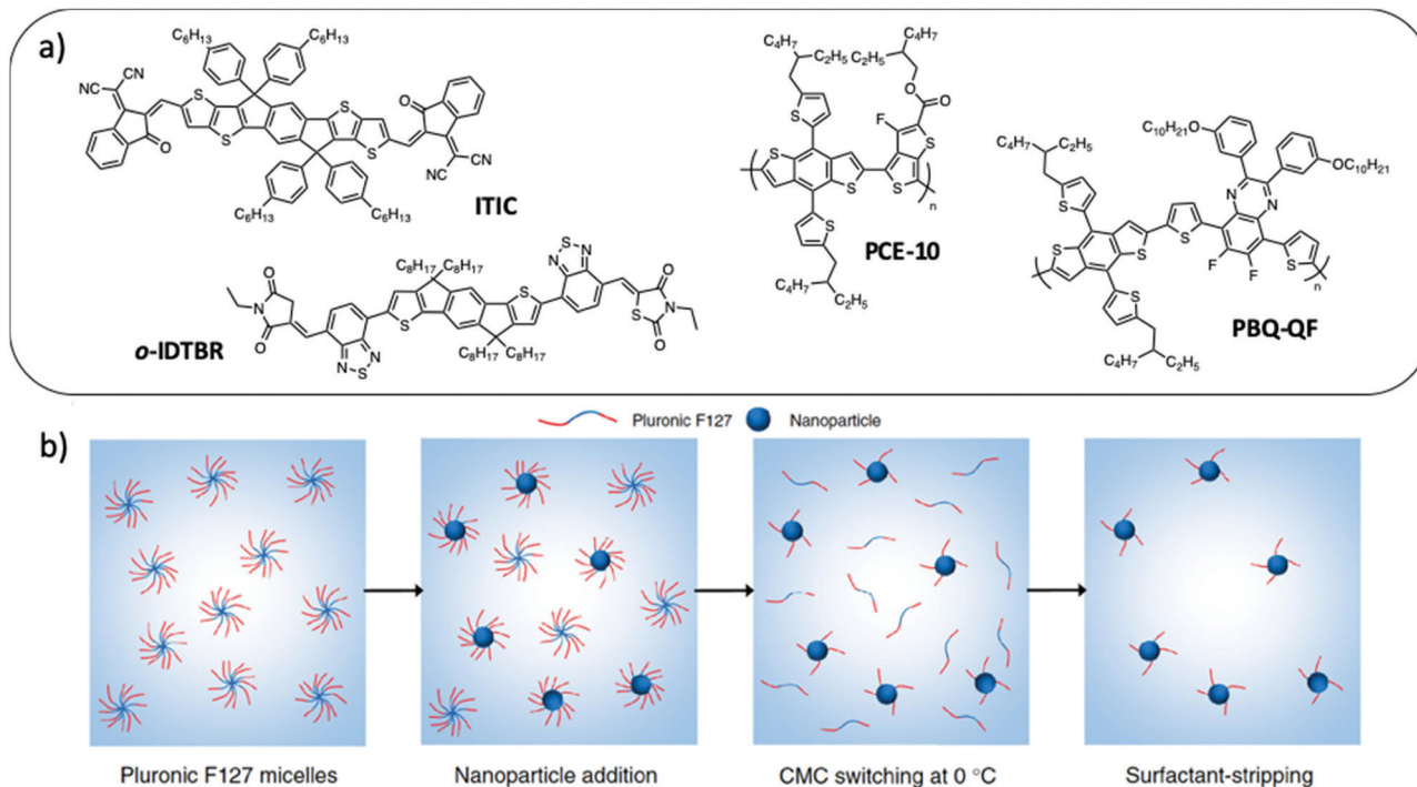
Fig. 10 (a) Chemical structures of ITIC, o -IDTBR, PCE-10 and PBQ-QF used to prepare NPs by surfactant-assisted nanoprecipitation. (b) Pluronic F127 is a copolymeric surfactant with a temperature-dependent critical micelle concentration (cmc). After elaboration of the NPs at room temperature, the dispersion is cooled down to 0 °C. At this low temperature, the surfactant becomes more soluble in water, its cmc increases and it desorbs from the NP surface. It can then be easily removed by centrifugal dialysis in a few steps only. Adapted with permission from ref. 49 (Copyright 2018 Springer Nature).
