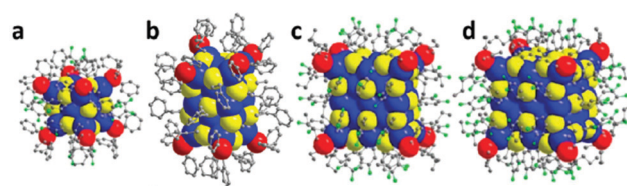
Fig. 5 X-ray structures of Ag cubes: Ag_{14}(SC_6H_3F_2)_{12}(PPh_3)_8 , Ag_{23}(PPh_3)_8(SC_2H_4Ph)_{18} , Ag_{38}(SPhF_2)_{26}(P^tBu_3)_8 , and Ag_{63}(SPhF_2)_{36}(P^tBu_3)_8 . Adapted with permission from ref. 62. Copyright 2019, Royal Society of Chemistry.
