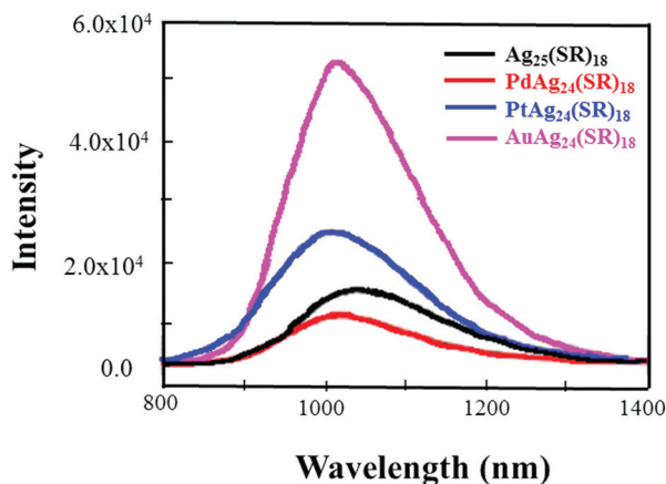
Fig. 27 PL spectra of \text{MAg}_{24}(\text{SR})_{18} ( \text{M} = \text{Ag/Pd/Pt/Au} ) NCs in the crystal state. Reproduced with permission from ref. 148. Copyright 2017, American Chemical Society.
