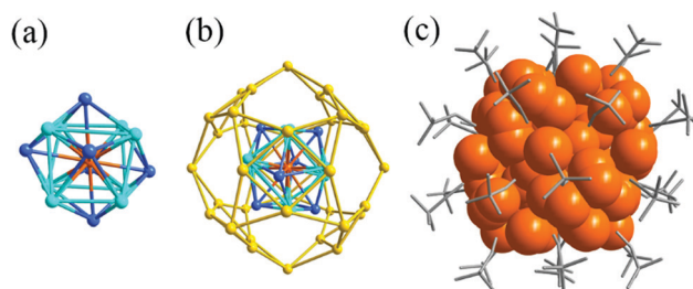
Fig. 16 (a) The \text{Ag}@Ag_{14} core; (b) the structure of the \text{Ag}@Ag_{14}@Ag_{36} shell; and (c) overall structure of \text{Ag}_{51}(\text{BuC}\equiv\text{C})_{32} . Adapted with permission from ref. 36. Copyright 2018, Royal Society of Chemistry.
