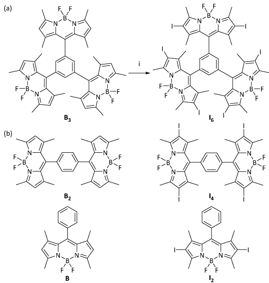
Fig. 1 (a) Synthesis of I 6 . Reactions conditions. (i) N -Iodosuccinimide, dichloromethane, 25 ^{\circ}\text{C} , 4 h. (b) Chemical structures of related BODIPY molecules reported elsewhere. 44,45
