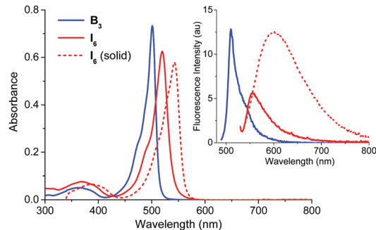
Fig. 2 Absorption and (inset) emission spectra of B 3 (6 \mu\text{M} ) and I 6 (4.5 \mu\text{M} ) in acetonitrile (solid lines) and that of I 6 in the solid state (dashed lines). The emission spectra were obtained by exciting the samples at the respective absorption maxima.
