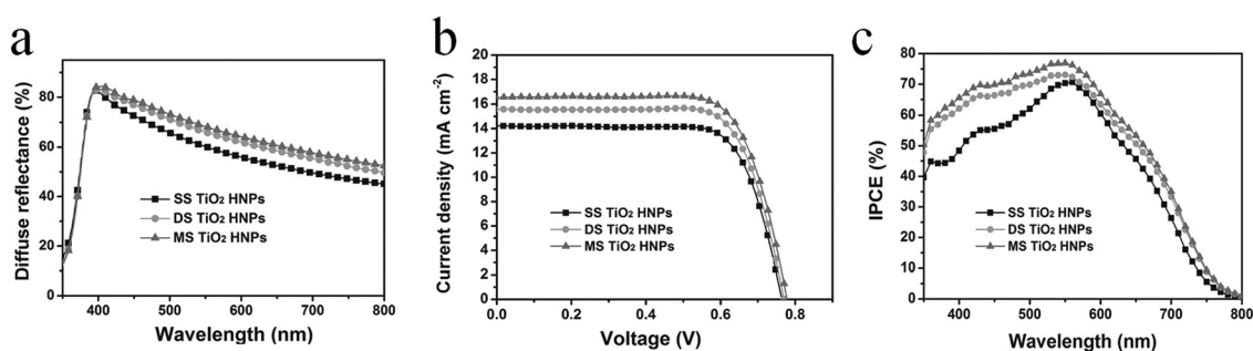
Fig. 41 (a) Diffuse reflectance spectra, (b) current density–voltage characteristics ( J–V curves), and (c) IPCEs of SS- \text{TiO}_2 -HNPs (square), DS- \text{TiO}_2 -HNPs (circle), and MS- \text{TiO}_2 -HNPs (triangle). Reprinted from ref. 22 with kind permission.
