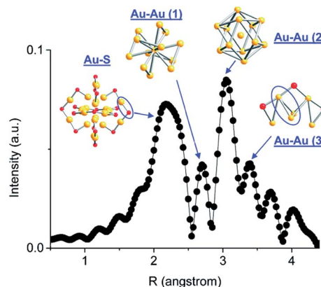
Fig. 2 Simulated FT-EXAFS of \text{Au}_{25}(\text{SR})_{18} clusters. The simulation was done by averaging the EXAFS from all representative Au sites of \text{Au}_{25} ( k : 3–14.5 Å −1 , k^4 weighted). The spectrum was phase-corrected using the Au–S peak. Reprinted with permission from ref. 43. Copyright 2011, American Chemical Society.
