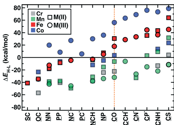
Fig. 8 Adiabatic gas phase spin splitting, \Delta E_{\text{H-L}} , in \text{kcal mol}^{-1} for octahedral complexes with \text{CO} and isoivalent or isoelectronic ligands. Complex energetics are shown for all converged DFT results in M(\text{II}) (squares) and M(\text{III}) (circles) oxidation states with \text{Cr} (gray), \text{Mn} (green), \text{Fe} (red), and \text{Co} (blue) metals. Ligands are ordered to be monotonically increasing for \text{Fe}(\text{II/III}) complexes, which are shown as solid red symbols, whereas all other metals and oxidation states are shown as translucent symbols to aid comparison. The metal coordinating atom in the ligand is underlined.
