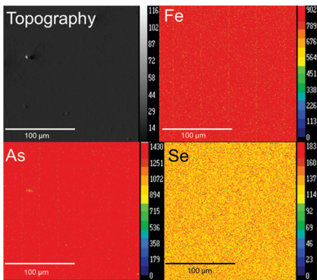
Fig. 3 Topological and X-ray elemental maps of single crystal \text{FeAs}_{1.50}\text{Se}_{0.50} from EMPA.
