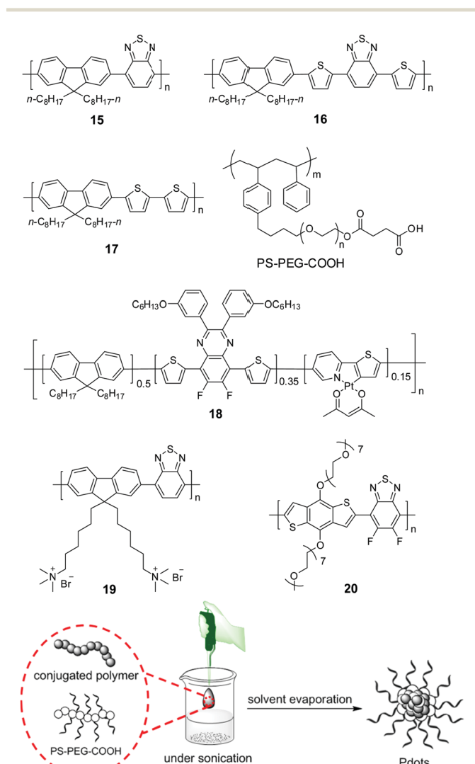
Fig. 6 Chemical structures of polymers 15–20 and preparation of polymer dots (Pdotes) by the nano-precipitation method for photocatalytic \text{H}_2 production. The scheme is adapted with permission from ref. 82, Copyright 2016 Wiley-VCH.
