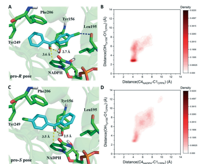
Fig. 7 Comparison of two critical distances between the pro- R and pro- S poses. The yellow dashed line represents the initial distance obtained in the docking results. The deeper red color represents the higher probability of the corresponding conformations. A. Docking result obtained for the pro- R pose. B. The probability density distribution of pro- R conformations obtained from the simulations. The conformations of pro- R binding demonstrated a close contact with NADPH and Tyr156 simultaneously. C. Docking result obtained for the pro- S pose. D. The probability density distribution of pro- S conformations obtained from the simulations. The conformations of pro- S binding demonstrate relatively dispersed distances to Tyr156 and NADPH.
