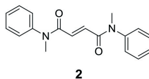
Fig. 1 Chemical structures of the compounds studied in this work.
