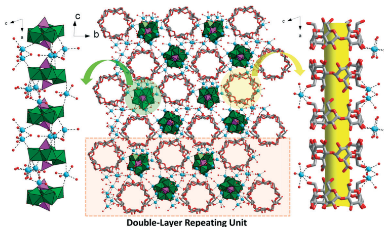
Fig. 2 Combined polyhedral/ball-and-stick representation of Na-PMo- \alpha -CD. Color code: MoO 6 , green octahedra; PO 4 pink tetrahedra; Na, turquoise; O, red; C, gray.
