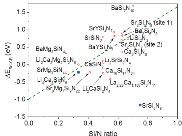
Fig. 7 \Delta E_{5d\text{-}CB} versus the Si/N ratio in the \text{Eu}^{2+} doped nitridosilicates. The straight line is a linear fit through the red data points. The blue squared data points represent exceptions discussed in the text.
