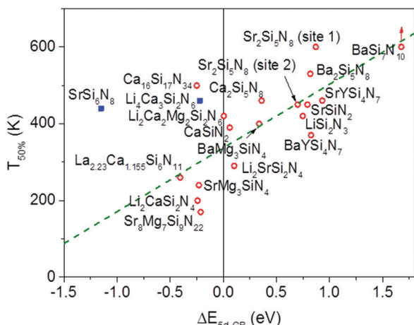
Fig. 6 Temperature at which 50% of the \text{Eu}^{2+} 5d–4f emission is quenched ( T_{50\%} ), versus the energy difference ( \Delta E_{5d\text{-}CB} ) between the bottom of the host lattice conduction band and the lowest \text{Eu}^{2+} 5d state. The straight green line is a linear fit through the red data points. The blue squared data points represent exceptions discussed in the text.
