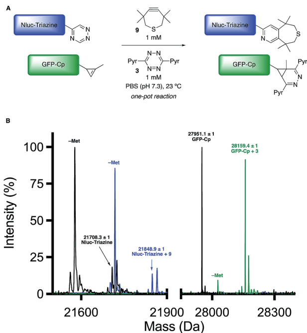
Fig. 5 Orthogonal [4 + 2] cycloadditions enable dual protein labeling. (A) Nluc-Triazine and GFP-Cp were mixed 1 : 1 in PBS (pH 7.3, 2 μM), and subsequently treated with TMTH (9) and tetrazine 3 (1 mM). (B) Quantitative conversion to the expected cycloadducts was observed after 3 h via mass spectrometry. N-Terminal methionine cleavage (-Met) was observed for both proteins and their respective cycloadducts.
