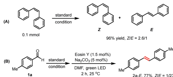
Scheme 4 Isomerization studies.
