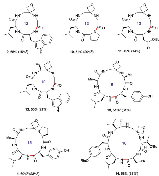
Fig. 3 Oxetane modified cyclic peptides by head-to-tail macrocyclisation. a,b Reaction conditions: DEPBT (2 equiv.), t Pr 2 EtN (2 equiv.), DMF (0.001 M), RT. b Bond formed in macrocyclisation indicated in red; yield in parenthesis for the cyclisation of linear peptide with C=O rather than oxetane in backbone. c PyBOP as activator. d Product isolated as the dimeric octapeptide. e DEPBT: 51%, d.r. >95 : 5; PyBOP: 64%, d.r. 3 : 1. f DMTMM tetrafluoroborate as activator. Data taken from ref. 13.
