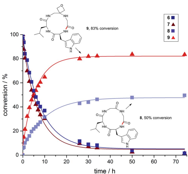
Fig. 2 Impact of oxetane modification on macrocyclisation rates: Cyclisation of WLGG ( 6 ) and oxetane modified WLGOxG ( 7 ) monitored over 74 h using DEPBT (2 equiv.), t Pr 2 EtN (2 equiv.) in DMF (0.001 M), RT. Bond formed in macrocyclisation indicated in red; peptides were quantified by analytical HPLC by integration of the corresponding UV signal at 280 nm (see ESI†).
