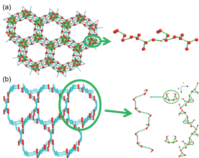
Fig. 17 1-D channels with water molecules in (a) \{[\text{Co}_3(m\text{-ClPhIDC})_2(\text{H}_2\text{O})_6] \cdot 2\text{H}_2\text{O}\}_n ( 1 ) and (b) \{[\text{Co}_3(p\text{-ClPhHIDC})_3(\text{H}_2\text{O})_3] \cdot 6\text{H}_2\text{O}\}_n ( 2 ). Red spheres represent O atoms in water, and green dots present H-bonding networks. Reproduced from ref. 74 with permission from American Chemical Society, Copyright 2017.
