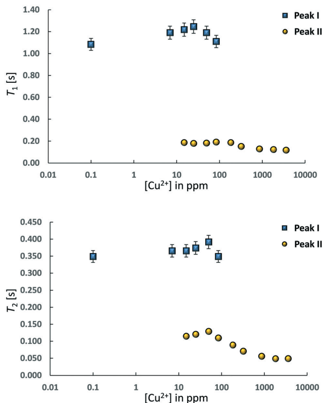
Fig. 3 T_1 and T_2 values for 1-octene in CuSO_4/Al_2O_3 samples at different concentration of CuSO_4 , expressed as [Cu^{2+}] . Peak I is associated to 1-octene interacting with Al_2O_3 whilst peak II is that of 1-octene interacting with CuSO_4 . The paramagnetic nature of Cu^{2+} ions leads to much smaller values of T_1 and T_2 NMR relaxation times of peak II.
