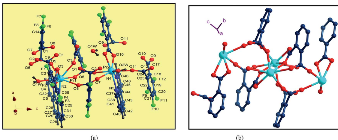
Fig. 1 (a) The coordination environments of Pr(III) ions in the asymmetric unit in 1 . (b) Diamond representation of tetranuclear clusters connected by carboxylic groups.
