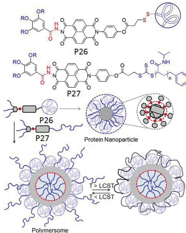
Fig. 29 (top) Structure of P26 and P27 . (bottom) Schematic representation of the supramolecular assembly of P26 and P27 (1 : 1). Adapted with permission from ref. 74. Copyright 2019, Wiley-VCH.
