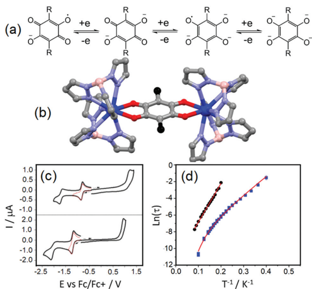
Fig. 1 (a) Electrochemical processes for tetraoxolene ligands. (b) Molecular structures of the dinuclear complexes 1 (R = Cl in black) and 2 (R = CH 3 in black). (c) Cyclic voltammograms of the yttrium analogues of 1 (up) and 2 (below). (d) Arrhenius plot of relaxation rates of 1 (blue squares) and 2 (black spots) in a 1600 Oe applied magnetic field with the best fits (red lines, see main text for descriptions). Colour code: carbon: grey, nitrogen: light blue, boron: pink, oxygen: red and dysprosium: blue. Adapted from ref. 20.
