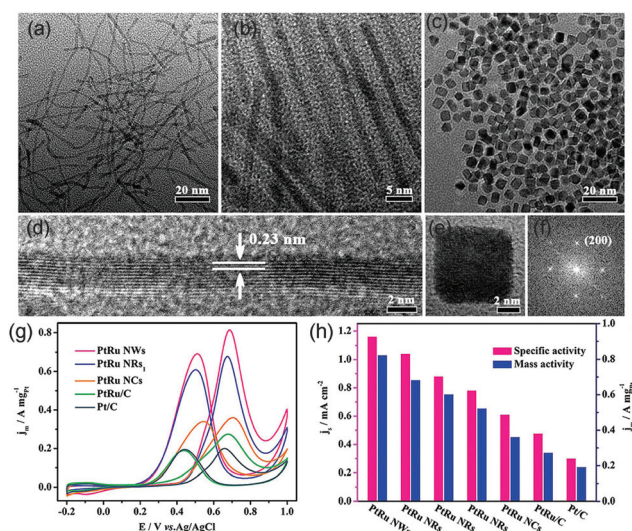
Fig. 15 TEM images of (a) PtRu NWs, (b) PtRu NRs 1 , and (c) PtRu NCs. HRTEM images of an individual (d) PtRu NW and (e) PtRu NC, and the corresponding FFT pattern (f) of (e). (g) Electrocatalytic performances of PtRu nanocrystals and commercial Pt/C catalysts. CVs of (g) PtRu NWs, PtRu NRs 1 , PtRu NCs, commercial PtRu/C, and commercial Pt/C for MOR in 0.1 M HClO 4 + 0.5 M CH 3 OH solution at a sweep rate of 50 mV s -1 . (h) Histograms of the mass and specific activities of different catalysts. Adapted with permission from ref. 187. Copyright 2017, American Chemical Society.
