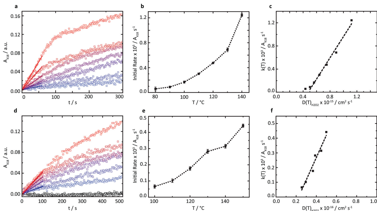
Fig. 4 (a) Plots of absorbance at 418 nm versus time indicating the production of DAP from 80 °C to 140 °C at 10 °C intervals (blue to red) in the cGOx-S 1 /cHRP-S 1 cascade. (b) Linear regression analysis of the two-enzyme cascade profiles (over 60 s) indicates a strong temperature dependence of initial reaction velocity. (c) Initial reaction velocity k(T) versus \text{H}_2\text{O}_2 diffusion coefficient D(T) is linear above 80 °C, indicating the production of DAP is diffusion-limited. (d) Plots of absorbance at 418 nm versus time indicating the production of DAP at 110 °C is inhibited in the cGOx-S 1 /cHRP-S 1 pair upon addition of acetyl-protected glucose (open black squares). Addition of cTLL-S 1 to the solvent-free biofluid re-initiates a three-enzyme cascade, as shown by the production of DAP from 100 °C to 150 °C at 10 °C intervals (blue to red). (e) Linear regression analysis of the three-enzyme cascade profiles (over 100 s) indicates a strong temperature dependence of initial reaction velocity. (f) Initial three-enzyme reaction velocity k(T) versus \text{H}_2\text{O}_2 diffusion coefficient D(T) is linear, indicating the production of DAP is diffusion-limited.
