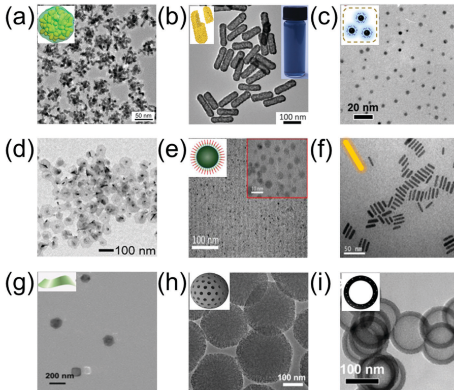
Fig. 2 TEM of (a) hyperbranched Au plasmonic blackbodies (AuPBs), (b) gold hollow nanorods (AuHNRs), (c) bismuth nanoparticles (Bi NPs), (d) \text{Bi}_2\text{Se}_3 nanoplates (NPs), (e) \text{CuS}@\text{BSA-RGD} NPs, (f) \text{Cu}_3\text{BiS}_3 nanorods (NRs), (g) \text{Cu}_2\text{MnS}_2 NPs, (h) mesoporous carbon nanospheres (Meso-CNs), and (i) black hollow silicon oxide nanoparticles (H- \text{SiO}_x NPs). (a) was reproduced from ref. 16 with permission from the American Chemical Society, Copyright 2018, (b) was reproduced from ref. 47 with permission from the American Chemical Society, Copyright 2018, (c) was reproduced from ref. 48 with permission from the American Chemical Society, Copyright 2017, (d) was reproduced from ref. 49 with permission from the Royal Society Chemistry, Copyright 2018, (e) was reproduced from ref. 50 with permission from the Royal Society Chemistry, Copyright 2018, (f) was reproduced from ref. 51 with permission from Elsevier Ltd, Copyright 2017, (g) was reproduced from ref. 52 with permission from Ivyspring International Publisher, Copyright 2017, (h) was reproduced from ref. 53 with permission from Ivyspring International Publisher, Copyright 2018 and (i) was reproduced from ref. 54 with permission from Elsevier Ltd, Copyright 2017.
