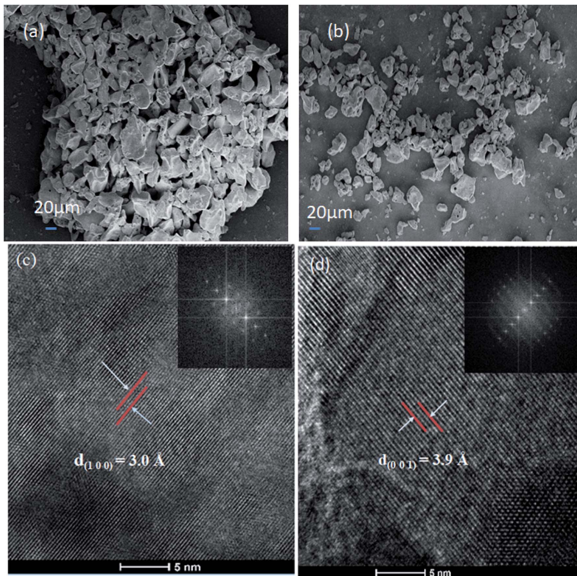
Fig. 7 (a) SEM image of \text{Nb}_2\text{O}_5 , (b) SEM image of \text{Sr} (0.25\%) - \text{Nb}_2\text{O}_5 , (c) HRTEM image of \text{Nb}_2\text{O}_5 showing the d spacing of the (1 0 0) plane and the inset shows the FFT image, and (d) HRTEM image of \text{Nb}_2\text{O}_5 showing the d spacing of the (0 0 1) plane and the inset presents the FFT image.
