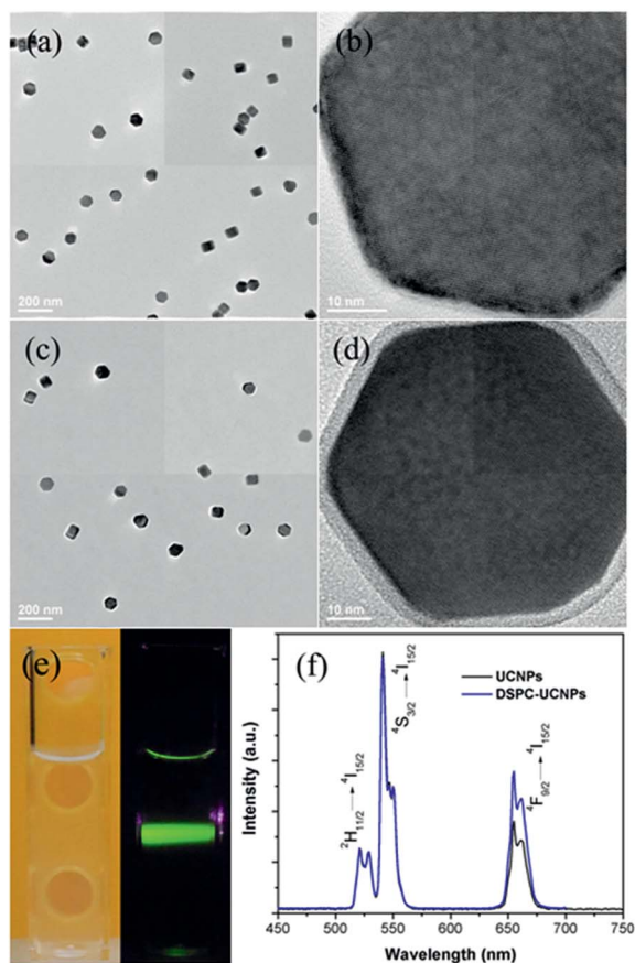
Fig. 4 TEM images of the (a and b) as-prepared and (c and d) phospholipid DSPC coated UCNPs deposited on a TEM grid from a drop of UCNPs cyclohexane solution and DSPC-UCNP water solution, respectively; (e) photographs of the water solution of DSPC-UCNPs without laser illumination and the upconverted visible luminescence under continuous-wave 980 nm laser illumination; (f) room-temperature UCL spectra of the as-prepared UCNPs in cyclohexane and DSPC-UCNPs in water under excitation at 980 nm.
