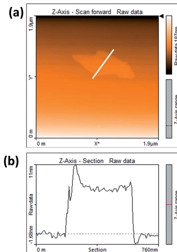
Fig. 3 (a) AFM image of \text{MoS}_2 nanosheets and (b) corresponding AFM height profile of \text{MoS}_2 nanosheets.
