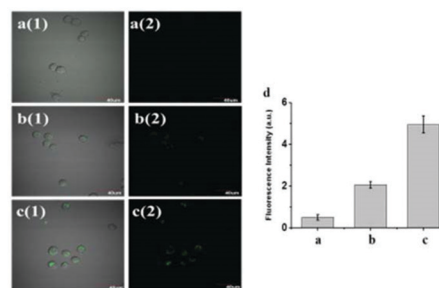
Fig. 106 Confocal fluorescence images of RAW 264.7 cells: (a) RAW 264.7 cells stained with 64 (5 \mu\text{M} ) for 15 min. (b) RAW 264.7 cells stimulated with 1 \mu\text{g mL}^{-1} LPS and 50 \text{ng mL}^{-1} IFN- \gamma for 4 h, and then 10 nM PMA for 30 min before incubation with 64 (5 \mu\text{M} ) for 15 min. (c) RAW 264.7 cells stained with 64 (5 \mu\text{M} ) for 15 min and then \text{ONOO}^- (10 \mu\text{M} ) was added for 20 min. (d) Relative fluorescence intensity of cells in panels (a)–(c). (1) Overlay field. (2) Green channel. Green channel: 460–540 nm, excitation at 404 nm. Copyright 2018 Royal Society of Chemistry.
