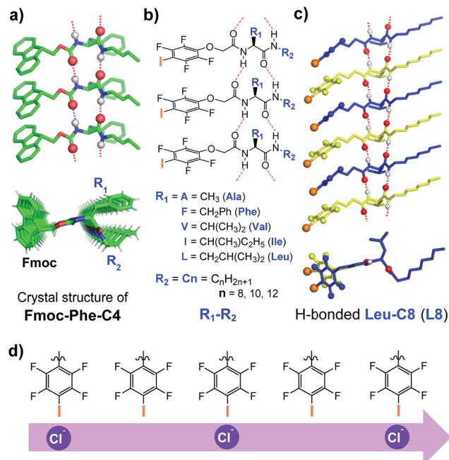
Fig. 1 (a) Crystal structure of F-Phe-C4, illustrating the formation of the 1D columnar stack with directionally assembled side chains. (b) Molecular design of the chloride-transporting channel library with systematically tunable R_1 and R_2 groups. (c) Side and top views of the computationally optimized H-bonded 1D columnar ensemble formed from L8. (d) A possible multi-ion jumping mode responsible for chloride transport.
