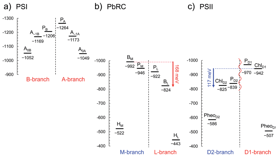
Fig. 2 E_m for one-electron reduction in the electron transfer chains in photosynthetic reaction centers of (a) PSI (PDB code 1JB0), (b) PbRC (PDB code 3I4D), and (c) PSII (PDB code 3ARC) in mV. Red and blue arrows indicate the E_m difference between accessory (B)Chla cofactors in PbRC and PSII, respectively. The red wavy line indicates the weak electronic coupling ( i.e. , uncoupling) between P_{D1} and P_{D2} . 49,50 Dotted lines indicate pseudo- C_2 axes. Electron-transfer active branches are red labeled, whereas inactive branches are blue labeled. See ref. 13 and 26 for calculated E_m values for one-electron oxidation in PSI, PbRC, and PSII.
