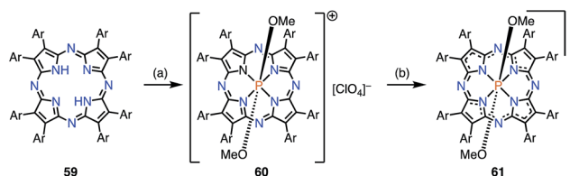
Fig. 19 Synthesis of 61 . (a) \text{POBr}_3 (200 equiv.), pyridine, 90^\circ\text{C} , 15 h, then \text{CH}_2\text{Cl}_2/\text{MeOH} , rt, 1 d. 60 was separated by \text{SiO}_2 column chromatography ( \text{CH}_2\text{Cl}_2/\text{MeOH}/\text{CF}_3\text{CO}_2\text{H} = 90/9.5/0.5 ), then \text{NaClO}_4 , \text{CH}_2\text{Cl}_2/\text{MeCN} , rt, 12 h, 56%; (b) 61 was separated by \text{Al}_2\text{O}_3 column chromatography (eluent: \text{CH}_2\text{Cl}_2/\text{TEA} = 99.5/0.5 ) without isolating 60 , 44%.
