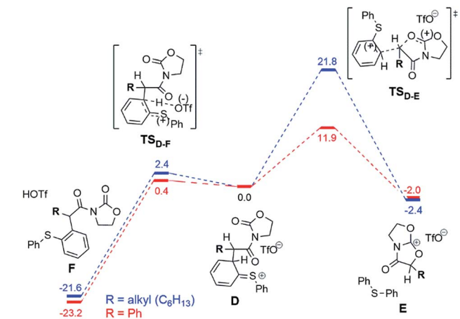
Fig. 7 Computed reaction profile (DFT, \Delta G_{298,\text{DCM}} ) for the conversion of the intermediate D into the main product F or the bicyclic cation E for the phenyl (red) and the alkyl (blue) substrates. The energy of the intermediate D is taken as a reference ( 0.0 \text{ kcal mol}^{-1} ).
