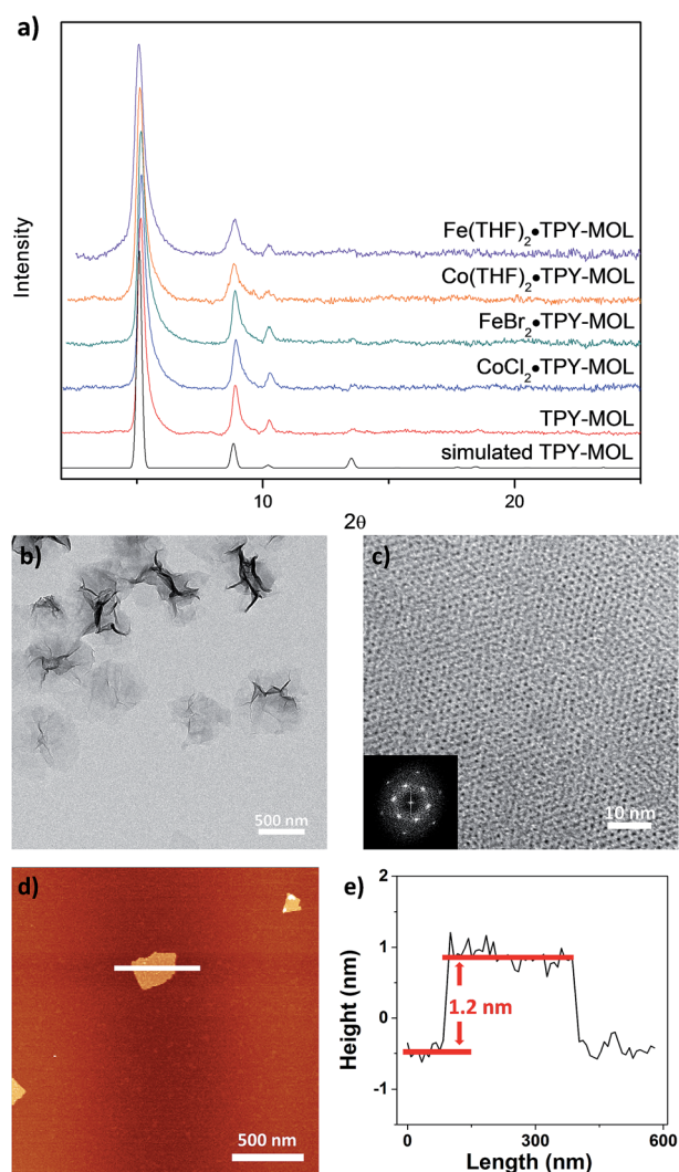
Fig. 2 (a) PXRD patterns of TPY-MOL, CoCl_2 \cdot TPY-MOL , FeBr_2 \cdot TPY-MOL , Co(THF)_2 \cdot TPY-MOL and Fe(THF)_2 \cdot TPY-MOL in comparison to simulated PXRD pattern for TPY-MOL; (b) TEM image of TPY-MOL; (c) HRTEM image and fast Fourier transform (FFT) pattern of TPY-MOL; (d) tapping-mode atomic-force microscope (AFM) topographic image of TPY-MOL; (e) height profile along the white line of TPY-MOL.
