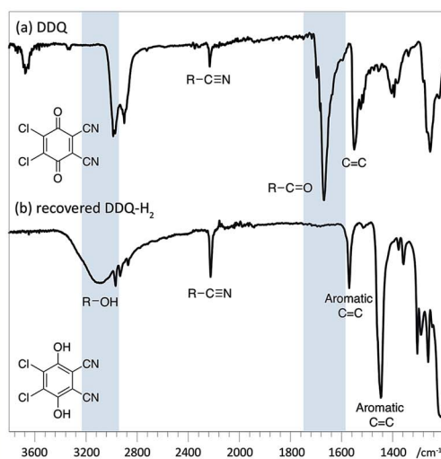
Fig. 8 Left: Recovery of DDQ-H 2 using celite packed fritted column (See Fig. S24 for colour image†). Right: IR spectra (cropped region) of (a) DDQ and; (b) recovered DDQ-H 2 . Characteristic differences in the spectra are highlighted with in blue.
