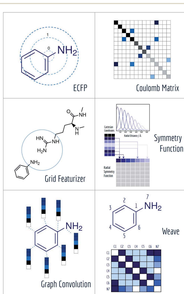
Fig. 5 Diagrams of featurizations in MoleculeNet.
