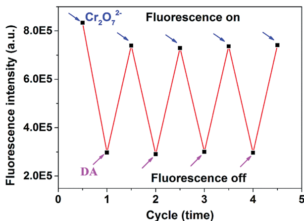
Fig. 6 Fluorescence intensity changes at 340 nm of PNCDs upon alternate addition of concentrations of 160 \mu\text{M} \text{Cr}(\text{vi}) and 160 \mu\text{M} DA in PBS (pH: 7.4).
