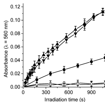
Fig. 3 Time course of NBT reduction as an increase in the absorption at \lambda = 560 nm in DMF/10% water. Samples contain NBT (0.2 mM), NADH (0.5 mM) and \text{TCP}-\text{C}_{60} (▲) (1.2 \mu\text{M} ) or \text{TCP}-\text{C}_{60}^{4+} (▼) (1.2 \mu\text{M} ) in DMF/10% water irradiated with light at \lambda_{\text{irr}} = 428 nm. Controls: NBT and NADH (●), \text{TCP}-\text{C}_{60} and NBT (Δ); \text{TCP}-\text{C}_{60}^{4+} and NBT (▽).
