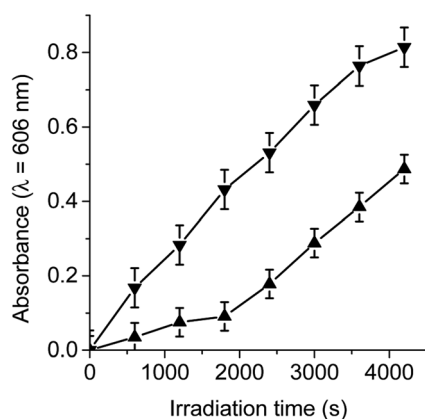
Fig. 2 Time course of \text{MV}^{2+} (0.8 mM) reduction as an increase in the absorption at \lambda = 606 nm sensitized by \text{TCP}-\text{C}_{60} (▲) (3.0 \mu\text{M} ) and \text{TCP}-\text{C}_{60}^{4+} (▼) (3.0 \mu\text{M} ) containing TMN (0.4 mM) after 10 min irradiation periods with light at \lambda_{\text{irr}} = 433 nm under an argon atmosphere in DMF/5% water.
