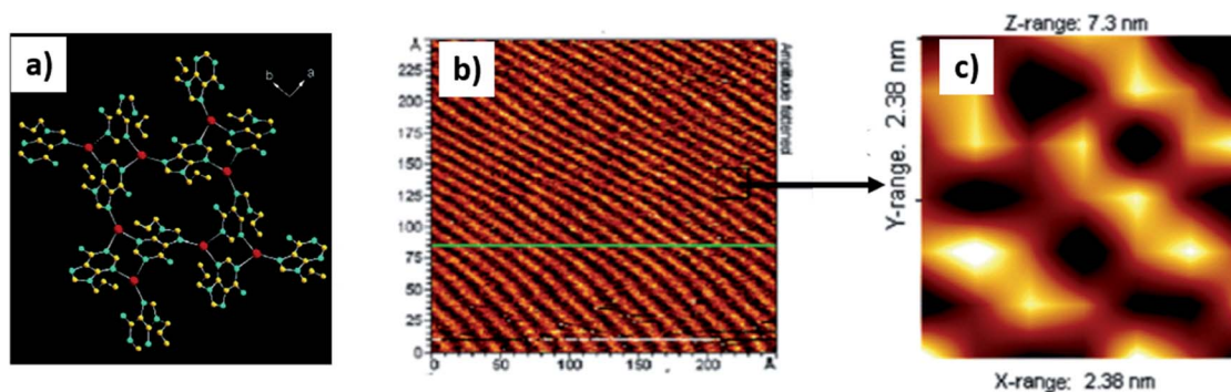
Fig. 23 (a) Adenine metallamacrocyclic complex 1. (b) AFM image of complex 1 on HOPG surface; (c) magnified image of (b) showing zig-zag assembly. (Reproduced with permission from ref. 117 © 2006 American Chemical Society).
