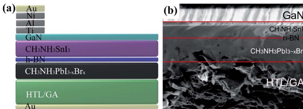
Fig. 2 (a) Cross-sectional schematic. (b) SEM images of perovskite cell with integral monolayer h-BN and graphene aerogel. 30
