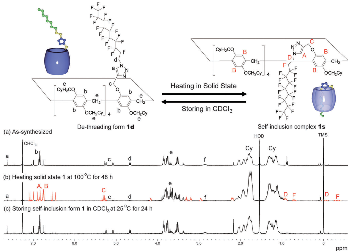
Fig. 2 ^1\text{H} NMR spectra of the host–guest conjugate 1 . As-synthesized (a), after heating of 1 in the solid state at 100 °C for 48 h, dissolving the solid sample in \text{CDCl}_3 , and obtaining the spectrum after 3 min (b), and 24 h (c).
