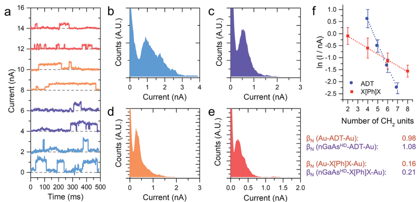
Fig. 3 (a) Example I(t) traces for n\text{GaAs}^{\text{HD}} – \text{X[Ph]X} –Au junctions. Traces are offset on the y axis for clarity. (b) Histogram constructed from 1154 individual current jumps for n\text{GaAs}^{\text{HD}} – 1[Ph]1 –Au junctions. (c) Histogram constructed from 532 individual current jumps for n\text{GaAs}^{\text{HD}} – 2[Ph]2 –Au junctions. (d) Histogram constructed from 1196 individual current jumps for n\text{GaAs}^{\text{HD}} – 3[Ph]3 –Au junctions. (e) Histogram constructed from 970 individual current jumps for n\text{GaAs}^{\text{HD}} – 4[Ph]4 –Au junctions. (f) Plot of current jump magnitude versus number of \text{CH}_2 units plot used to determine the value of \beta_N . All data shown in this Figure is obtained in the dark.
