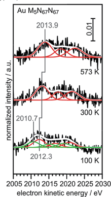
Fig. 7 XPS and X-ray excited Auger spectra of 0.02 ML Au/30 ML MgO (a) and 0.02 ML Au/3 ML MgO (b) for different annealing temperatures (bottom: 100 K; middle: 300 K; top: 573 K).
