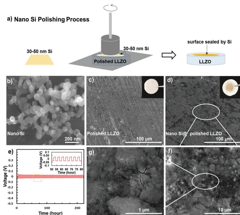
Fig. 6 (a) Schematic diagram of the nano Si polishing process and SEM images of (b) the nano-Si, (c) the surface of the polished LLZO (inset: digital image of the polished LLZO pellet), (d) the surface of the nano Si polished LLZO (inset: digital image of the nano-Si polished LLZO pellet) and enlarged images (f and g). (e) Cyclic performance of the Li/SSE/Li symmetric cell at room temperature with nano-Si polished LLZO as the SSE (inset: enlarged cycles between 50 and 80 hours), current density: 0.1 \text{ mA cm}^{-2} .
