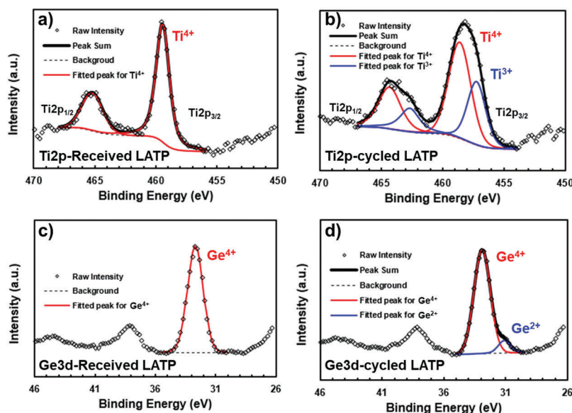
Fig. 4 XPS results of Ti 2p (a and b) and Ge 3d (c and d) of the LATP before and after cycling in the Li/LATP/Li symmetric cell.
