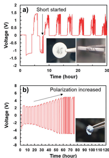
Fig. 1 Cyclic performance of (a) Li/LLZO/Li and (b) Li/LATP/Li symmetric cells at room temperature with a 0.1 \text{ mA cm}^{-2} current density. Inset: Digital photographs of (a) the surface and cross section of the cycled LLZO and (b) the surface of the cycled LATP (the cross section of the cycled LATP is not shown, as it is too thin to be seen with a digital camera).
