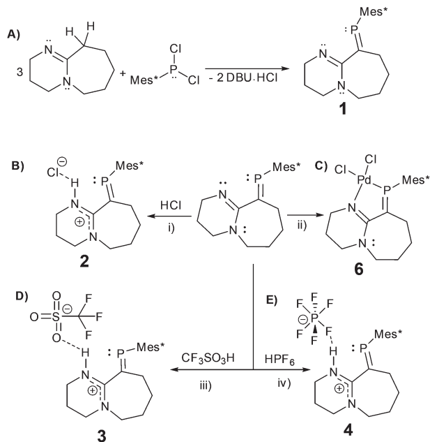
Scheme 2 Simplified synthetic procedures: (A) 1 ; THF, -78\text{ }^{\circ}\text{C} (B) 2 ; (i) anhydrous HCl (2 M, THF), THF, -78\text{ }^{\circ}\text{C} . (C) 6 ; (ii) [Pd(MeCN) 2 Cl 2 ], DCM, rt. (D) 3 ; (iii) CF 3 SO 3 H (neat), MS (3 Å), THF, -78\text{ }^{\circ}\text{C} . (E) 4 ; (iv) HPF 6 (60% aq.), MS (3 Å), THF, -78\text{ }^{\circ}\text{C} .
