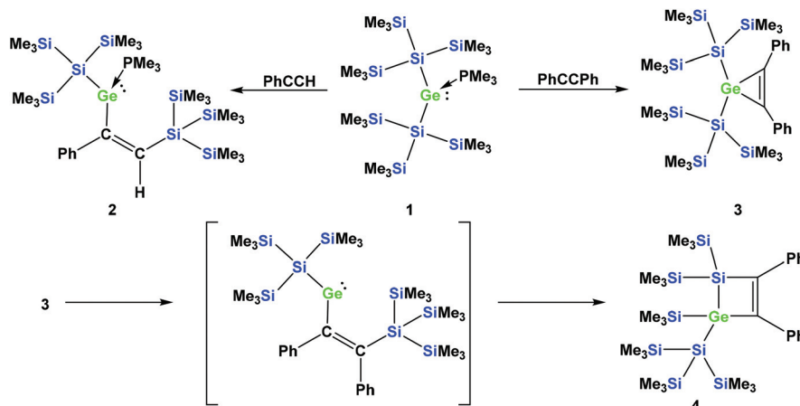
Scheme 1 Reactions of germylene adduct 1 with either phenylacetylene (top left) or tolane (top right). Thermally-induced rearrangement of germirene 3 to silgermacyclobutene 4 (bottom part).
