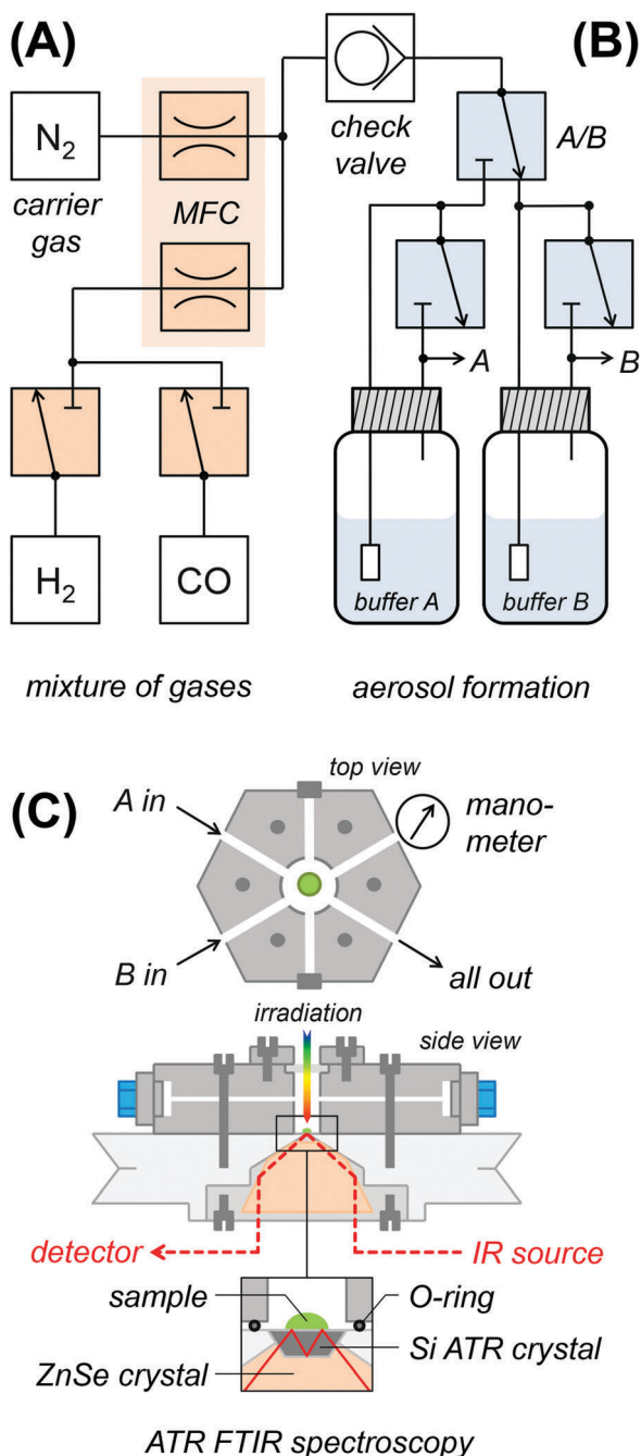
Fig. 2 Experimental set-up for ATR FTIR on protein films. (A) Various gases (e.g. H_2 , CO ) were mixed into a constant stream of N_2 carrier gas. The gas flow was controlled by digital mass flow controllers (MFC). (B) Dry gas was passed through either wash bottle A or B, comprising different buffer compositions. (C) The thereby created aerosol was fed to the headspace above the protein film. On top of the ATR reflection unit, a custom-made PCTFE chamber with gas in- and outlets and manometric pressure control capped the silicon crystal and the protein film.
