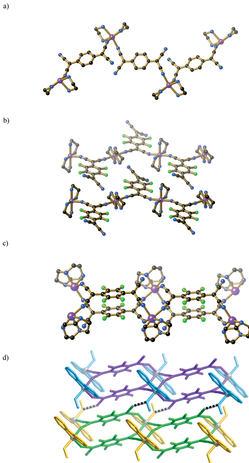
Fig. 1 1D coordination polymers in which divalent metal ions are linked by X_4TCNQ^{2-} ligands: a) a single chain of [Mn(en)_2(TCNQ)] (1) b) interdigitating chains of [Mn(en)_2(F_4TCNQ)] (2) c) a "double-layered" polymer of [Cd(TACN)(F_4TCNQ)] (4) and d) a pair of "double-layered" polymers of [Zn(F_4TCNQ)(2,2bipy)(MeOH)] (6) with hydrogen bonding between the chains indicated by striped connections.
