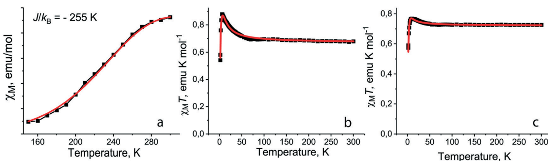
Fig. 7 (a) Temperature dependence of molar magnetic susceptibility of 1 in the 150–300 K range (black squares) and fitting the data by the Heisenberg model for quasi-square layered arrangement of spins 38 with J/k_B = -255 K (red curve); fitting the experimental \chi_M T data (black squares) by the modified S-T model 39 for 5 (b) with J_{\text{intra}}/k_B = +5.6 K, \theta = -1.4 K, g = 2 (fix), f = 0.996 (red curve) and for 7 (c) with J_{\text{intra}}/k_B = +3.3 K, \theta = -2.3 K, g = 2 (fix), f = 0.999 (red curve).
