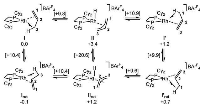
Scheme 10 Computed mechanisms for fluxionality and D-label scrambling in [1-( propene )][BAr F 4 ] in the solid-state. Gibbs free energies are indicated in kcal mol -1 with those for transition states provided in square brackets.
